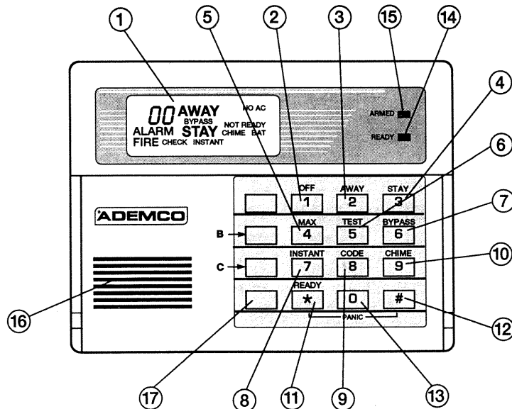
STYLE B CONSOLE
