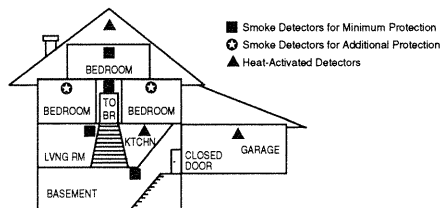
MAXIMUM FLOOR COVERAGE- DETECTORS AT TOP OF STAIRWELLS
